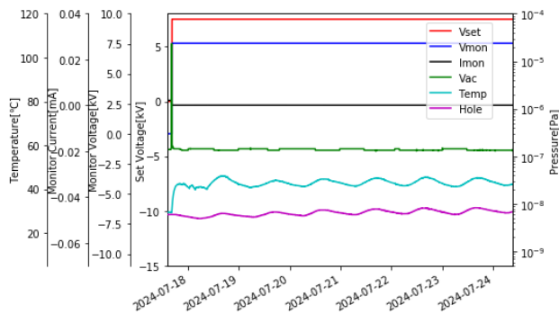
Figure 5: 2nd mass production prototype Continuous operation history (2024/7/17~2025/7/24).
