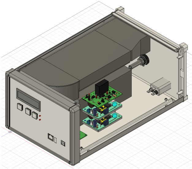
Figure 8: High current output ion pump power supply concept diagram.
