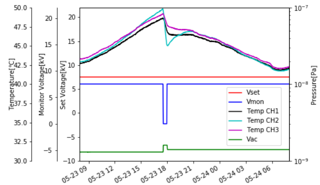
Figure 3: 1st mass production prototype thermostat operation history (2024/5/23~2024/5/24).
