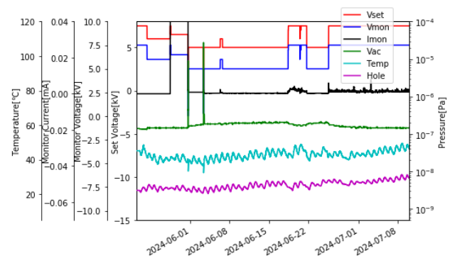
Figure 4: 1st mass production prototype Continuous operation history (2024/5/23~2025/7/10).
