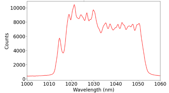
Figure 5: Spectrum of the 0th order light from the Yb fiber laser oscillator. The spectral width and center wavelength are 37 nm and 1033 nm, respectively.
