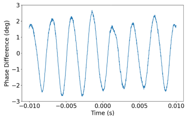
Figure 6: Phase difference signal from phase detector.
