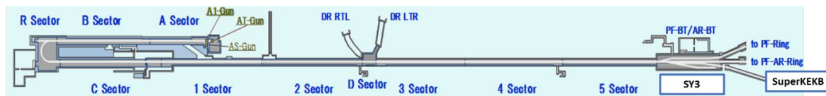
Figure 2: Layout of the KEK electron/positron injector linac.
