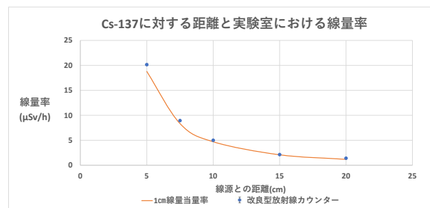
Figure 2: Variations in the dose rate as a function of a distance between the radiation source (Cs-137) and the measurement system in the laboratory.
