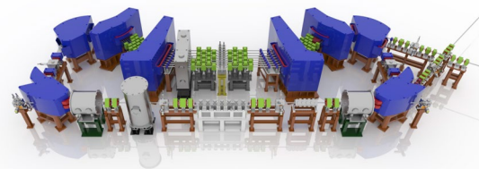
Figure 1: 3D design drawing of the CSR. Our final plan is to install two CSRs, CSR1 and CSR2.
