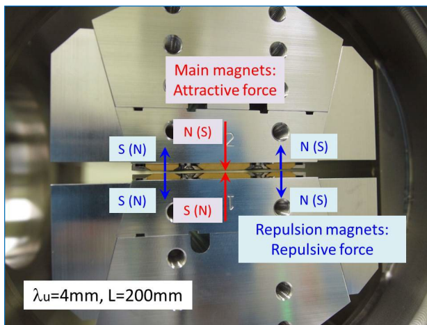
Figure 5: Magnet arrangement to cancel the magnetic attractive force between the main magnet arrays. The attractive force of the main magnets is cancelled by the repulsive force produced by the repulsive magnets arranged at both sides of the main array. A case for 4-mm period length is shown.
