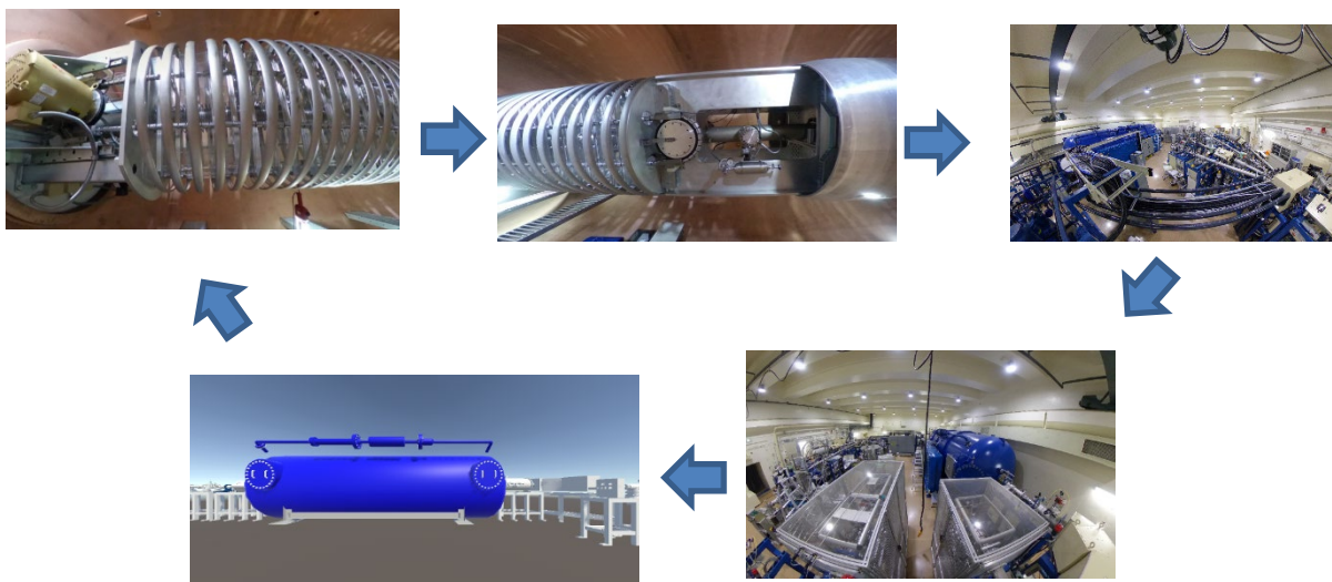
Figure 5: VR view of the 6MV Pelletron tandem accelerator.
