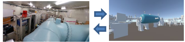
Figure 4: VR view of the 1MV Tandetron accelerator.
