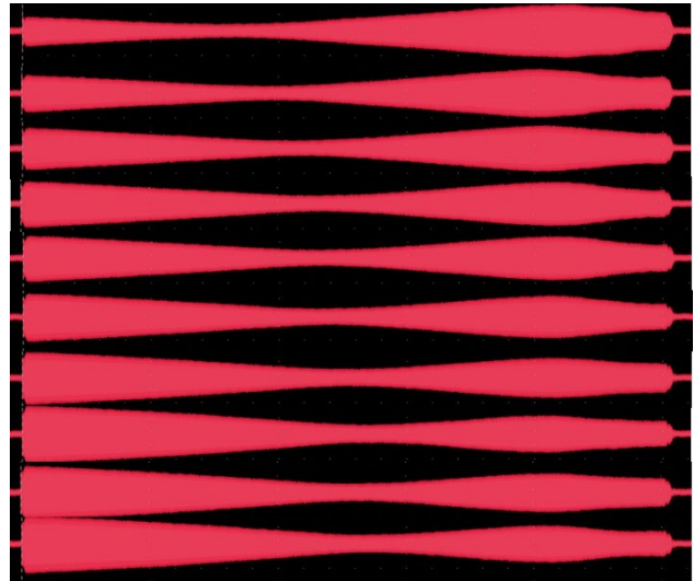
Figure 3: REV pulse shape for FWD = 220 kW, PW = 1 ms, RP = 20 ms; From top to bottom the cavity tuner is linearly swept to change cavity resonant frequency by a total of \sim 30 kHz.
