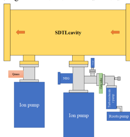
Figure 3: Measurement system.
