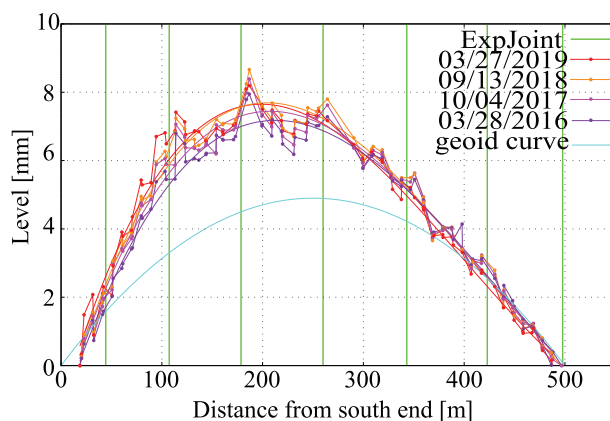
Figure 4: Evaluated the earth curvature with several years of QPD data are compared. The geoid curve (light blue) with the earth radius of 6371 km is also overlaid. Locations of expansion joints are represented as green lines.
