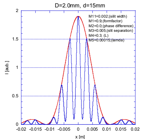
Figure 3: Calculated interferogram with double-slit (Blue line). Red line shows the sinc function. ( a = 2.0 mm, d = 15 mm, visibility = 0.9)
