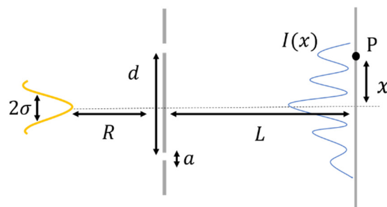
Figure 1: Beam size measurement using double slit.
