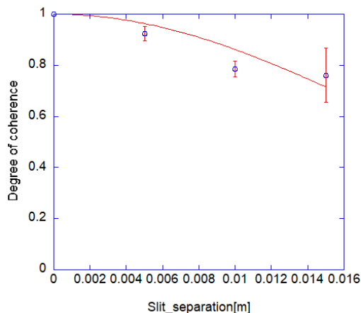
Figure 6: Measured degree of coherence as a function of slit separation.
