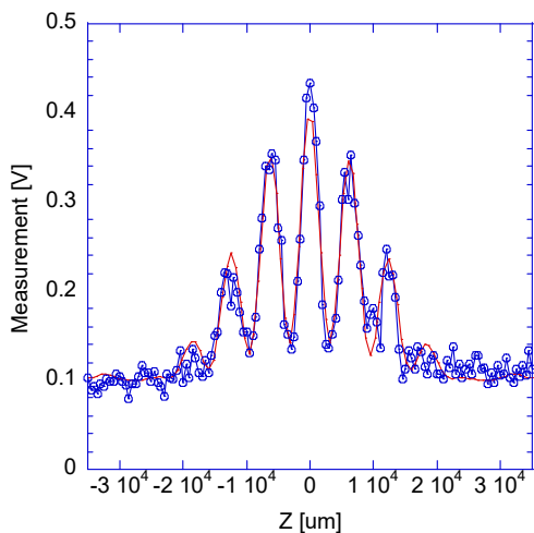
Figure 4: Horizontal Interferogram with double slit. ( a = 2.0 mm, d = 10 mm)
