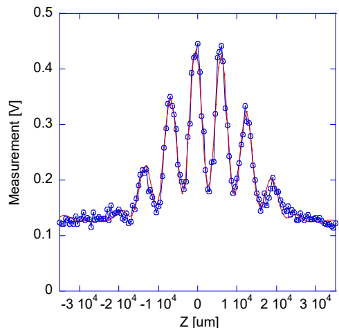
Figure 5: Vertical Interferogram with double slit.
