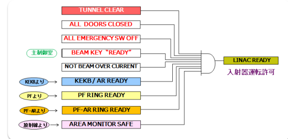
Figure 1: Block diagram of LINAC safety system interlock signal logic.
