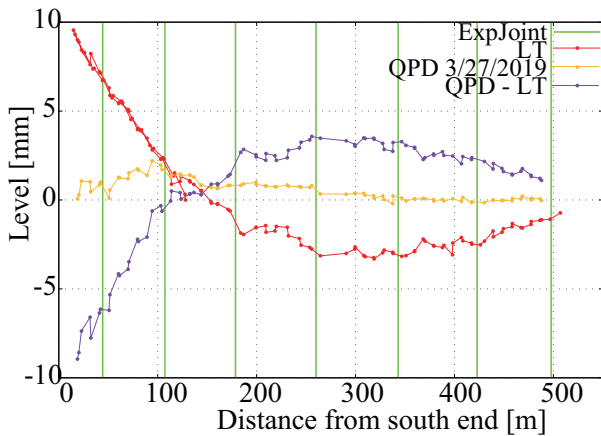
Figure 2: Level data of QPD (orange) and LT (red) are compared. Residuals of QPD and LT are also overlaid (purple). Locations of expansion joints are represented as green lines.
