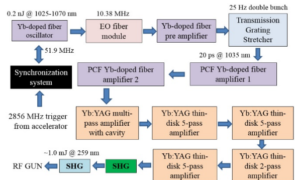
Figure 1: Layout of current laser system for RF-gun.
