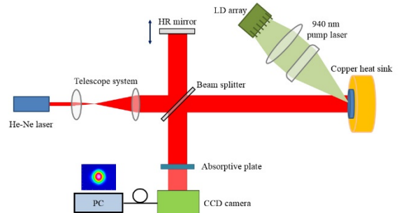
Figure 4: Optical measurement experimental setup.
