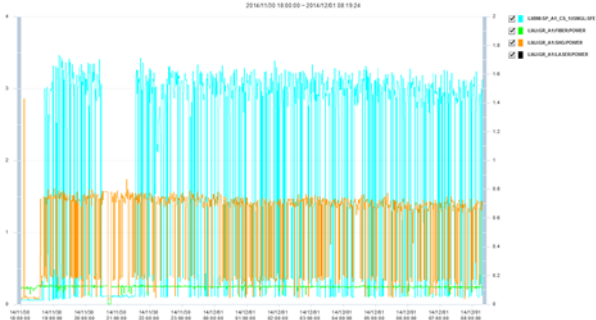
Figure 6: Electron bunch charge history.
