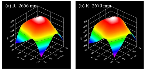
Figure 8: Wavefronts from Yb:YAG/Cu composite. (a) unpumped; (b) pumped.
