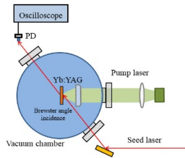
Figure 9: Gain test experimental layout.
