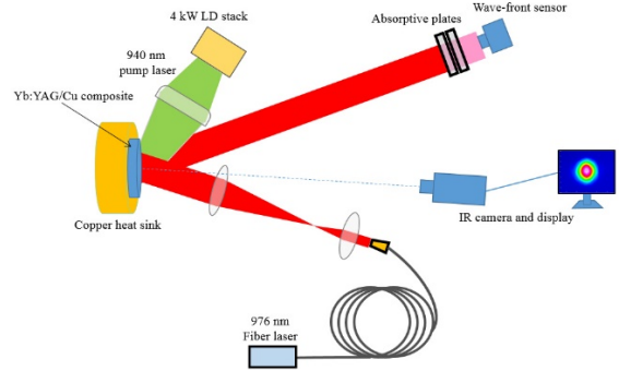
Figure 7: Measuring experimental setup of this disk deformation.
