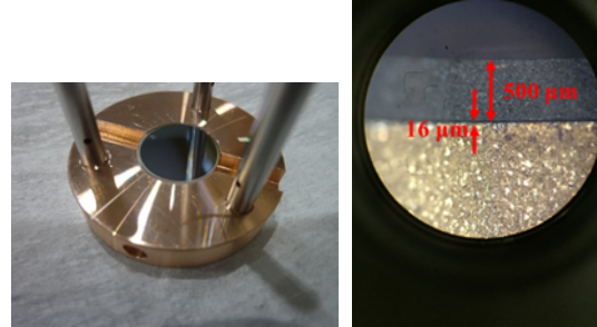
Figure 3: Accomplished Yb:YAG/Cu composite and side view under microscope.
