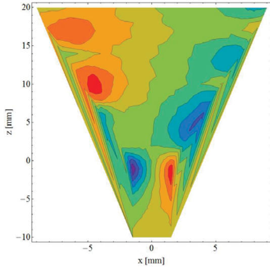
Figure 8: Contour plot of the transverse magnetic field B_x in xz plane for spiral slit FC.
