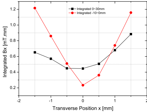
Figure 9: Integrated transverse magnetic field B_x along z for spiral slit FC.
