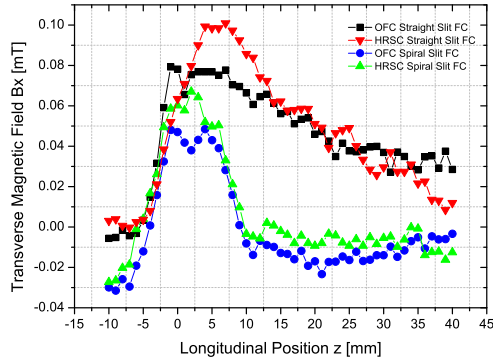
Figure 5: Transverse magnetic field B_x as a function of longitudinal position z for four FC prototypes. Black: OFC straight slit FC, red: HRSC straight slit FC, blue: OFC spiral slit FC and green: HRSC spiral slit FC.
