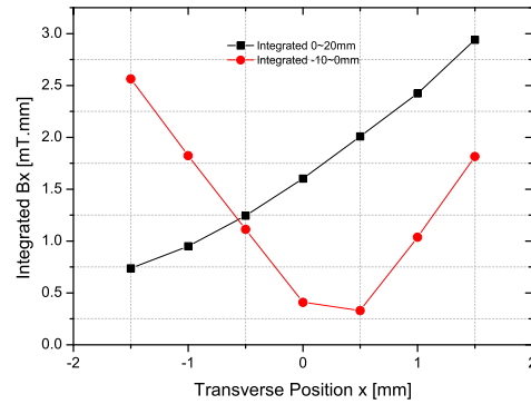
Figure 7: Integrated transverse magnetic field B_x along z for straight slit FC.
