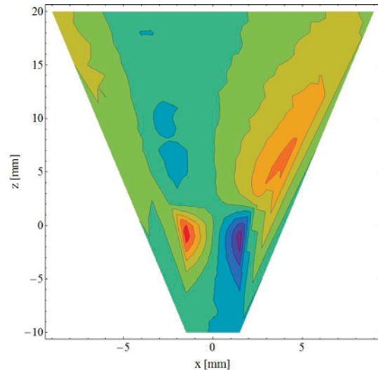
Figure 6: Contour plot of the transverse magnetic field B_x in xz plane for straight slit FC.
