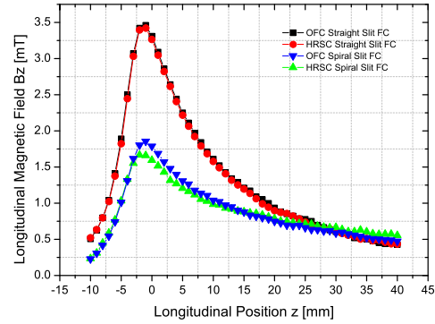
Figure 4: Longitudinal magnetic field B_z as a function of longitudinal position z for four FC prototypes. Black: OFC straight slit FC, red: HRSC straight slit FC, blue: OFC spiral slit FC and green: HRSC spiral slit FC.
