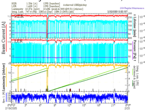
Figure 1: Typical KEKB operation in one day. Each graph shows the stored current of HER (top), LER (middle) and luminosity (bottom), respectively.
