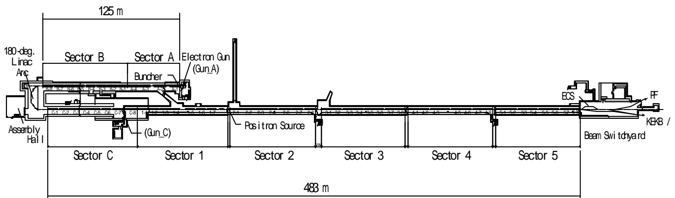
Figure 1: Layout of the KEKB injector linac. J-arc section combines two straight sections.
