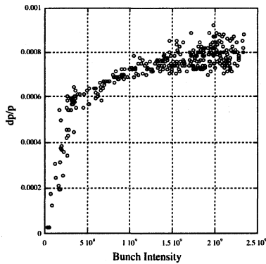
Fig. 4 The energy spread: measured at the extraction line beam profile monitor
