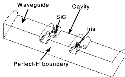
Figure 2: The drawing of single cavity for HFSS simulation
