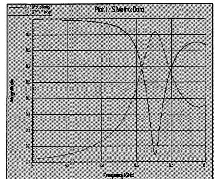
Figure 3: Typical S Matrix plot for S_{11} and S_{21} from HFSS.
