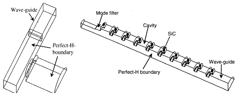
Figure 6: Drawing of impedance matching model for HFSS simulation; a) between rectangular wave-guide and mode filter and b) between the mode filter and the cavity-chain.
