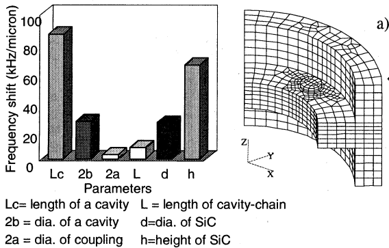
Figure 4: Frequency sensitivity of the TM_{011} cavity Figure 5: Thermal analysis of the TM_{011} main body using NASTRAN V70;
