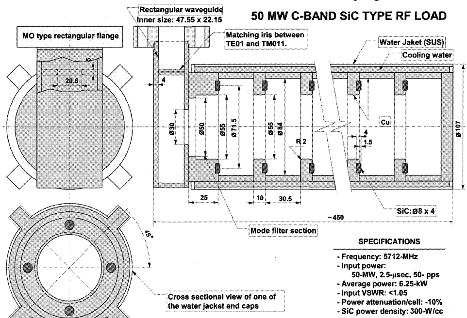
Figure 1: A conceptual drawing of 50-MW Class SiC rf-load.
