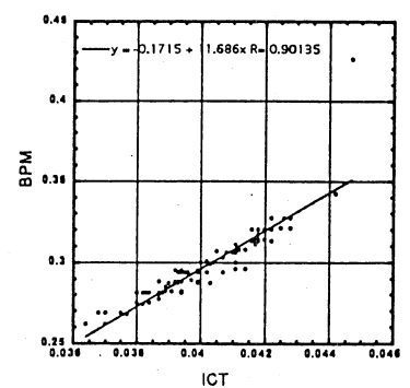
Fig. 3c) ICT-BPMsingle correlation
