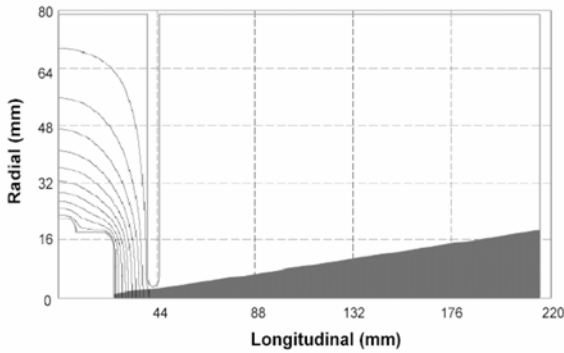
Figure 6: Extraction of an electron beam of 300 mA in a DC electron gun according to a simulation with EGUN.
