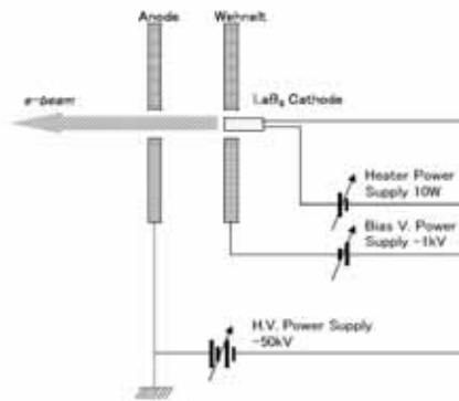
Figure 1: The schematic diagram of DC gun system.
