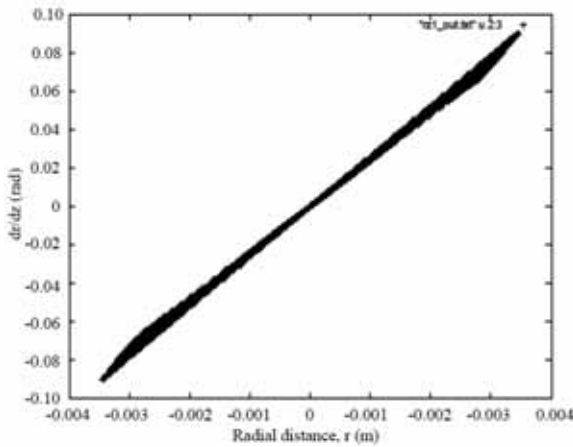
Figure 7: The phase space distribution at 1 cm from the anode exit according to a simulation with EGUN.
