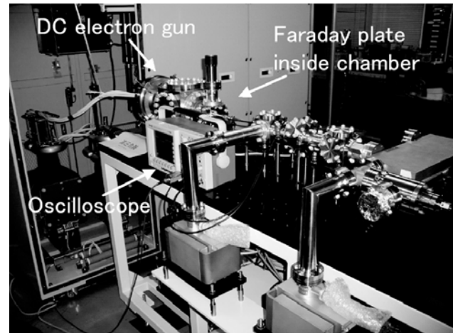
Figure 4: The measurement of gun voltage and beam current.
