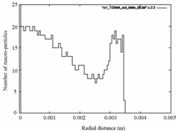
Figure 8: The macro-particle distribution at 1 cm from the anode exit according to a simulation with EGUN.
