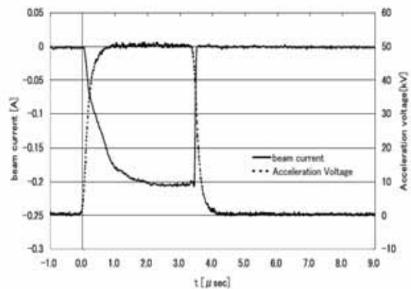
Figure 5: The waveform of accelerating voltage and beam current.
