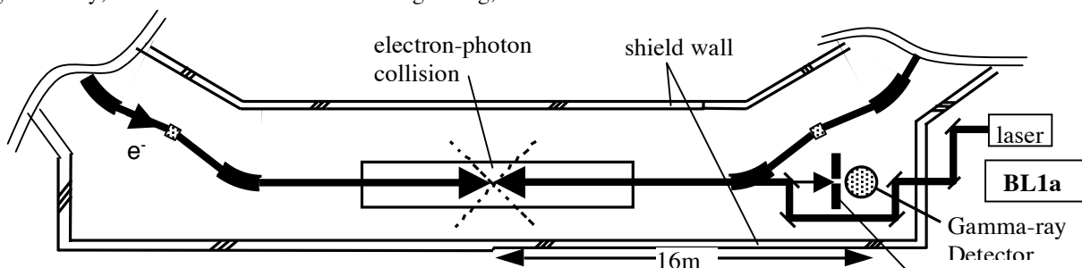
Fig.3 BL1, laser-Compton gamma ray experimental area. Laser was injected from the outside of the wall.
