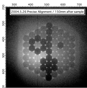
Fig.5 Gamma-ray radiography image. Sample targets are bundle rods of Al and Au with 2mm in diameter and 50mm in length.
