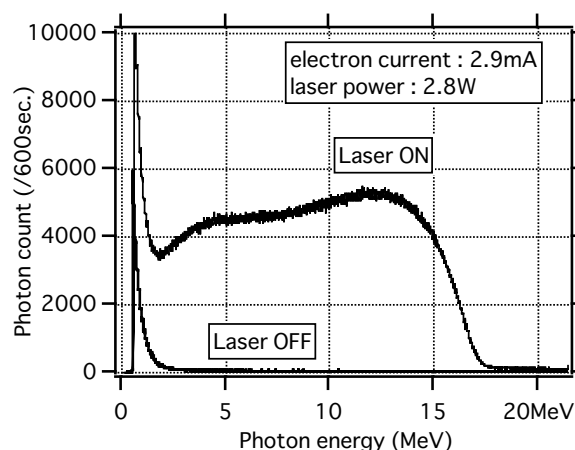
Fig.4 Examples of the laser Compton gamma ray signal. Pb collimator of 24mm in diameter was used.
