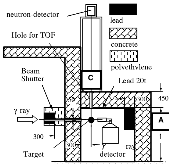
Fig.6 Shielding design of the laser Compton gamma-ray beam-line (BL1)
