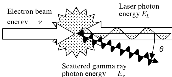
Fig.1 Laser Compton scattering gamma-ray generation.
