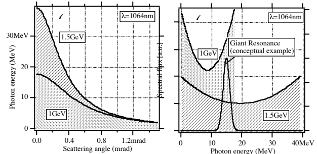
Fig.2 Spectral characteristics of Laser Compton scattering gamma ray on NewSUBARU (1 to 1.5 GeV) with a laser of 1064 nm wavelength. (a) Angular distribution of gamma ray. (b) Spectral distribution of gamma ray compare with spectral cross-section of giant resonance of photo nuclear reaction.
