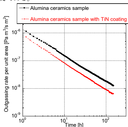
Figure 8: Measured outgassing rate per unit area of alumina ceramics. The measurement result of alumina ceramics with TiN coating is also shown.
