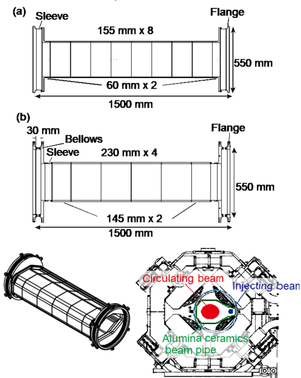
Figure 2: Configuration of the (a) existent and (b) newly designed alumina ceramics beam pipes for the injection quadrupole magnet. Position relation to the magnet is also shown.
