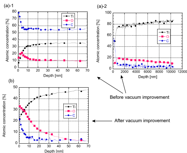
Figure 5: AES depth profile on Ti surface after treatment of brazing condition (a) without and (b) with vacuum improvement.
