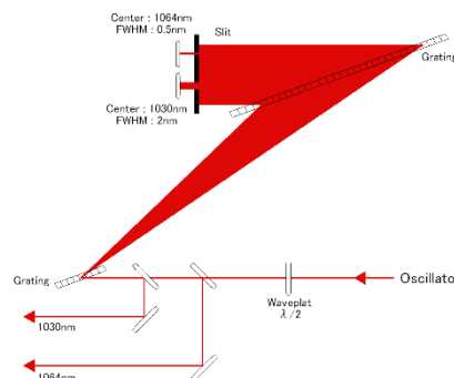
Figure 7: Grating stretcher.
