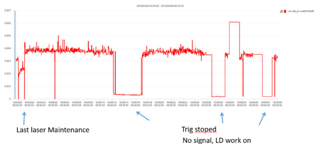
Figure 2: Stability of Laser system from 4/26 to 6/9.
