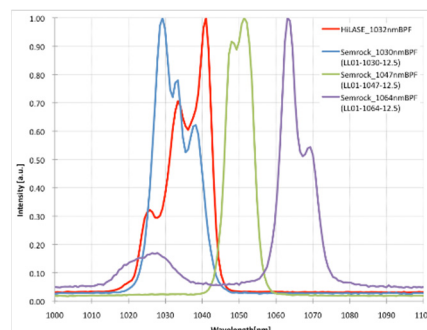
Figure 6: The spectrum of the oscillators.
