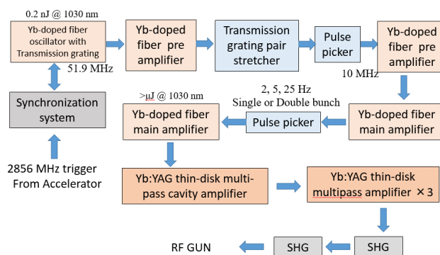
Figure 1: Layout of Laser system.
