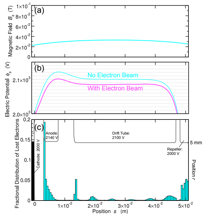
Figure 5: Simulation results for prototype ion source: (a) Axial magnetic field along s -axis, (b) Potential distribution along s -axis, and (c) Lost electron distribution and electrode structure. The lost electron distribution is normalized by total number of emitted electrons. Electrons reflected by the repeller are not taken into account.
