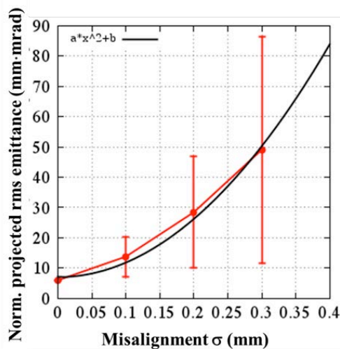
Figure 2: Vertical emittance at the end of the 5-sector as a function of magnitude of misalignment.
