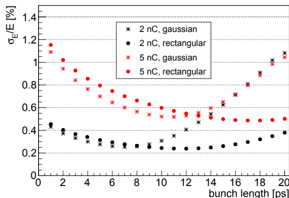
Figure 7: Energy spread at the end of the 5-sector as a function of bunch length with on-crest RF phase.
