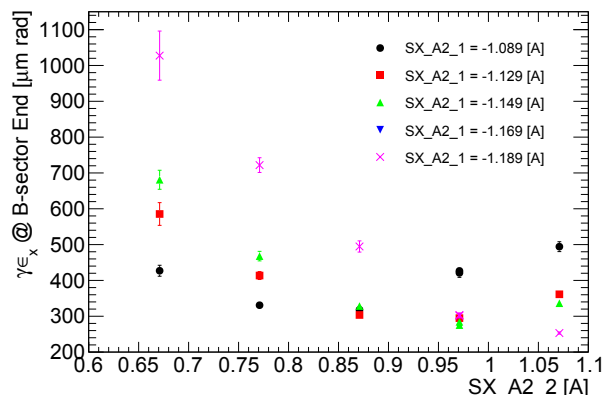
Figure 6: Horizontal emittance as a function of currents in two steering coils placed at the start of the A-sector.
