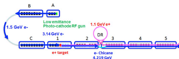
Figure 1: Schematic of SuperKEKB injector linac.
