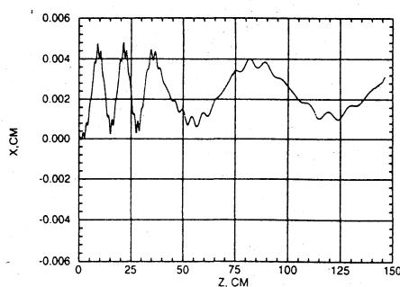
Fig. 4. Oscillation of center mass of the beam due to vanes asymmetry of \Delta = 50 microns.
