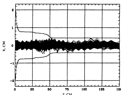
Fig. 3. Particle trajectories in the RFQ structure with the error in vane fabrication of \delta = 50 microns (see result 2 in Table 2). Transmission efficiency is 92%.
