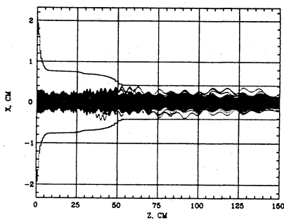
Fig. 2. Particle trajectories in RFQ structure (see results 1,2,3 in Table 1). Transmission efficiency is 94%.
