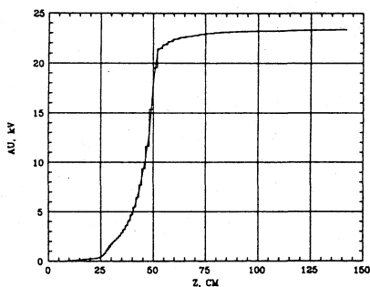
Fig. 1. Linear (PARMTEQ-type) and step-wise function of axial voltage at every cell along the RFQ structure.
