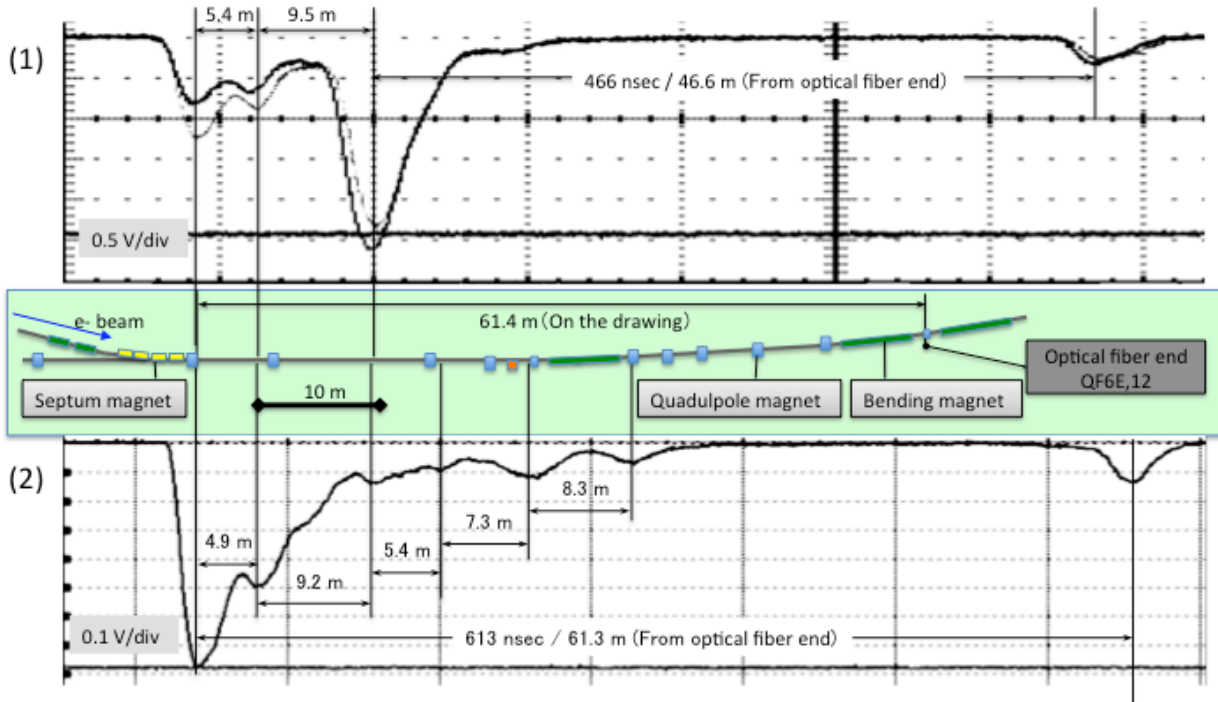
Figure 3: Schematic of a magnet on a part of beam injector and waveform of HER beam loss monitor.
