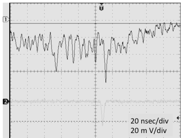
Figure 10: Waveform of wire scanner.
