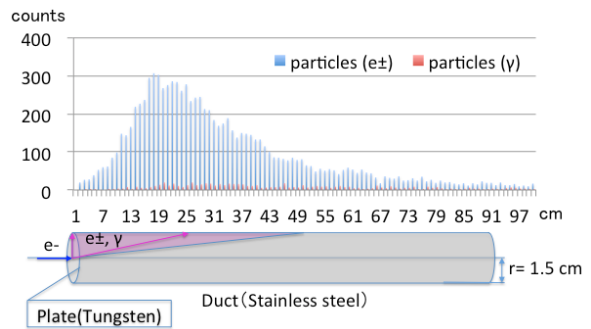
Figure 9: Histogram of the particle when the energy of the incident beam is 45 MeV.
