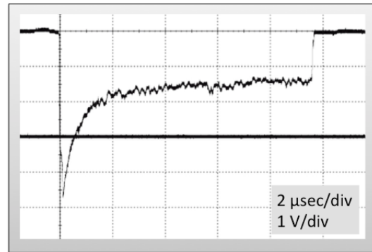
Figure 5: Waveform of the beam loss monitor when a HER beam has aborted.
