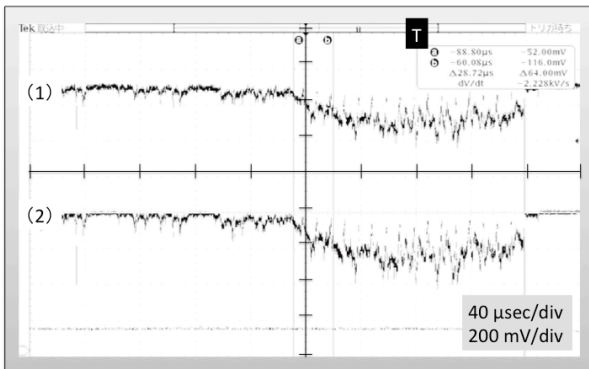
Figure 7: Waveform of the beam loss monitor when a LER beam has aborted.
