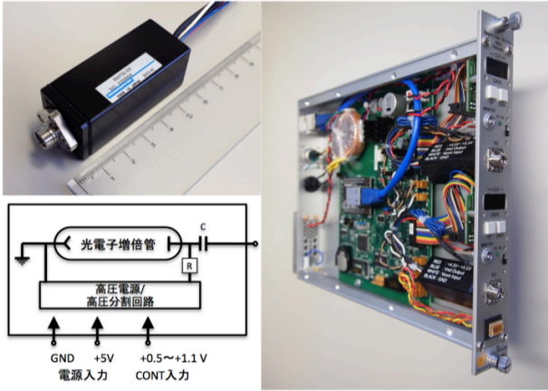
Figure 2: Beam Loss Monitor Module.
