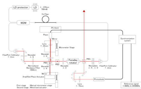
Figure 5: ANDi type Oscillator.
