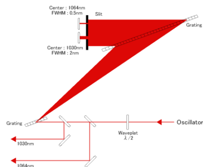
Figure 7: Grating stretcher
