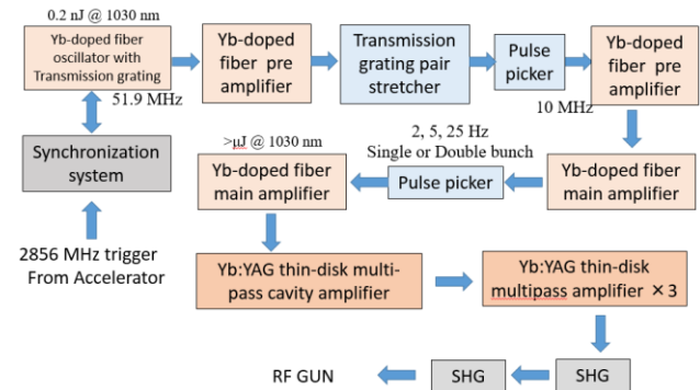
Figure 1: Layout of Laser system.
