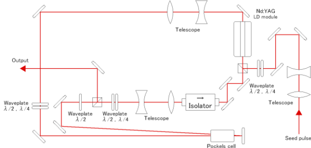
Figure 8: Nd:YAG Rod regenerative amplifier
