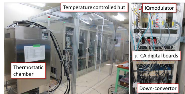
Figure 2: LLRF control racks.
