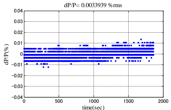
Figure 10: Stability of beam energy. (After improvement)
