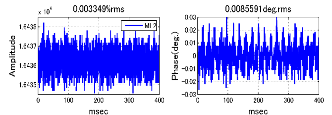
Figure 5: Stability of ML2: 0.0033% rms in amplitude and 0.0086° rms in phase.
