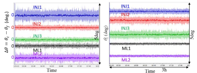
Figure 9: Stabilities of detuning angles \Delta\theta (left) and cavity phases \theta_c (right). (After improvement)
