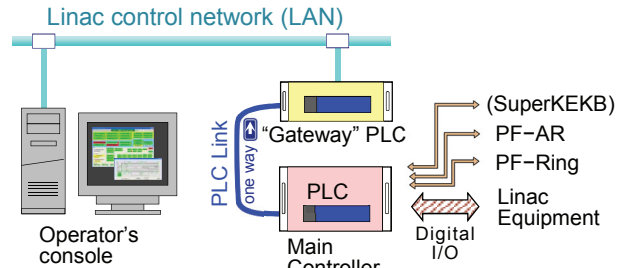
Figure 2: A rough view of Linac interlock system layout.
