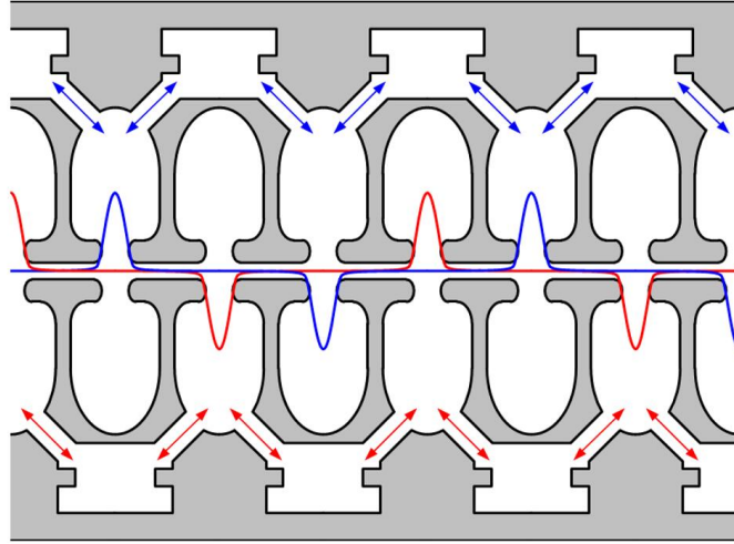
Figure 11.63: Quasi-travelling wave generated by the side coupled cavities.
