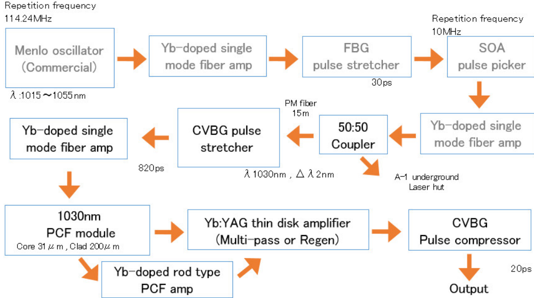
Figure 11.77: Layout of Underground laser system.
