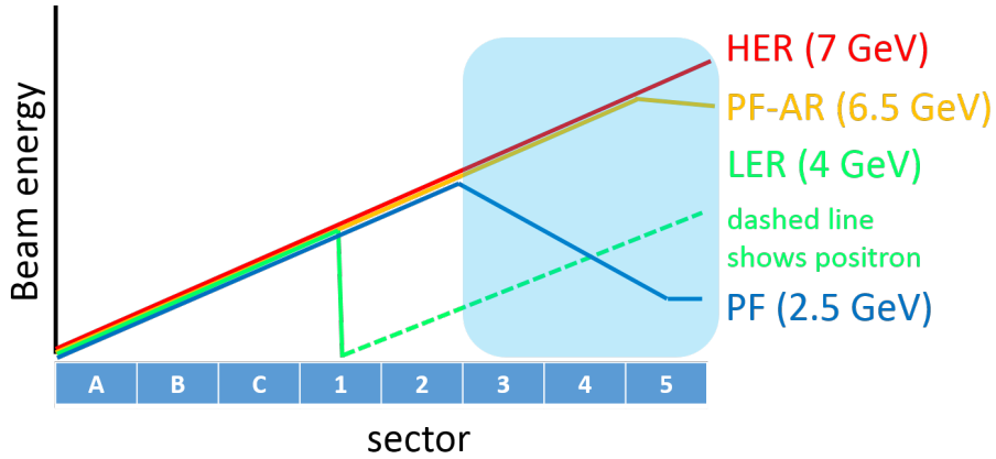
Figure 11.37: Beam energy along the beam line. Solid line shows electron beam dashed line shows positron beam respectively.
