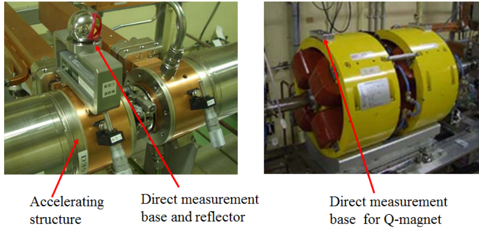
Figure 11.51: Direct position measurement point with laser tracker for all relevant hard wares.
