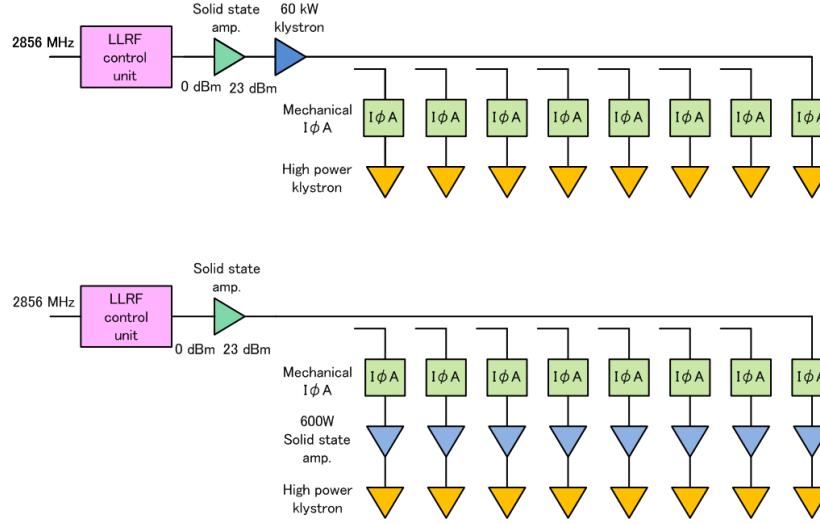
Figure 11.26: Diagram of the sub-booster system in the KEKB injector linac (up) and planned for Sthe SuperKEKB injector linac (down).
