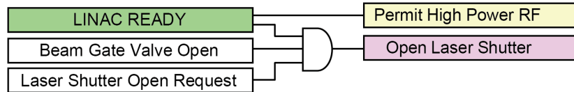
Figure 11.103: Requirements for operating the RF gun.
