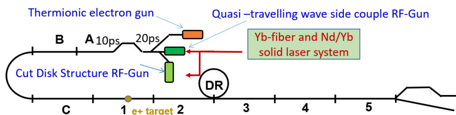
Figure 11.4: Layout of RF-gun and thermionic electron gun.
