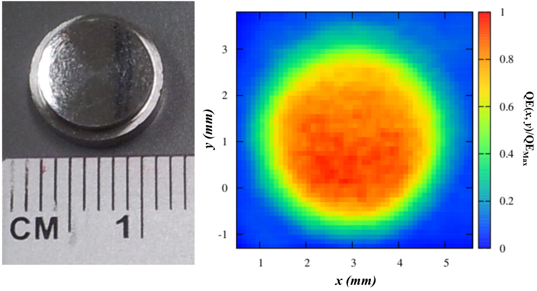
Figure 11.69: \text{Ir}_7\text{Ce}_2 photocathode and the measured quantum efficiency map.
