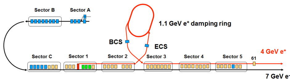
Figure 11.12: Linac schematic of acceleration unit configuration.
